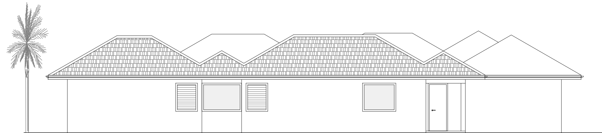
02 SIDE (WEST) ELEVATION NO SCALE
